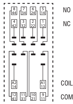
ACCESSORY Metallic retainer RC4-N Marker - SRN-BM-1 Plug-in modules PDME1 to RPDME1
